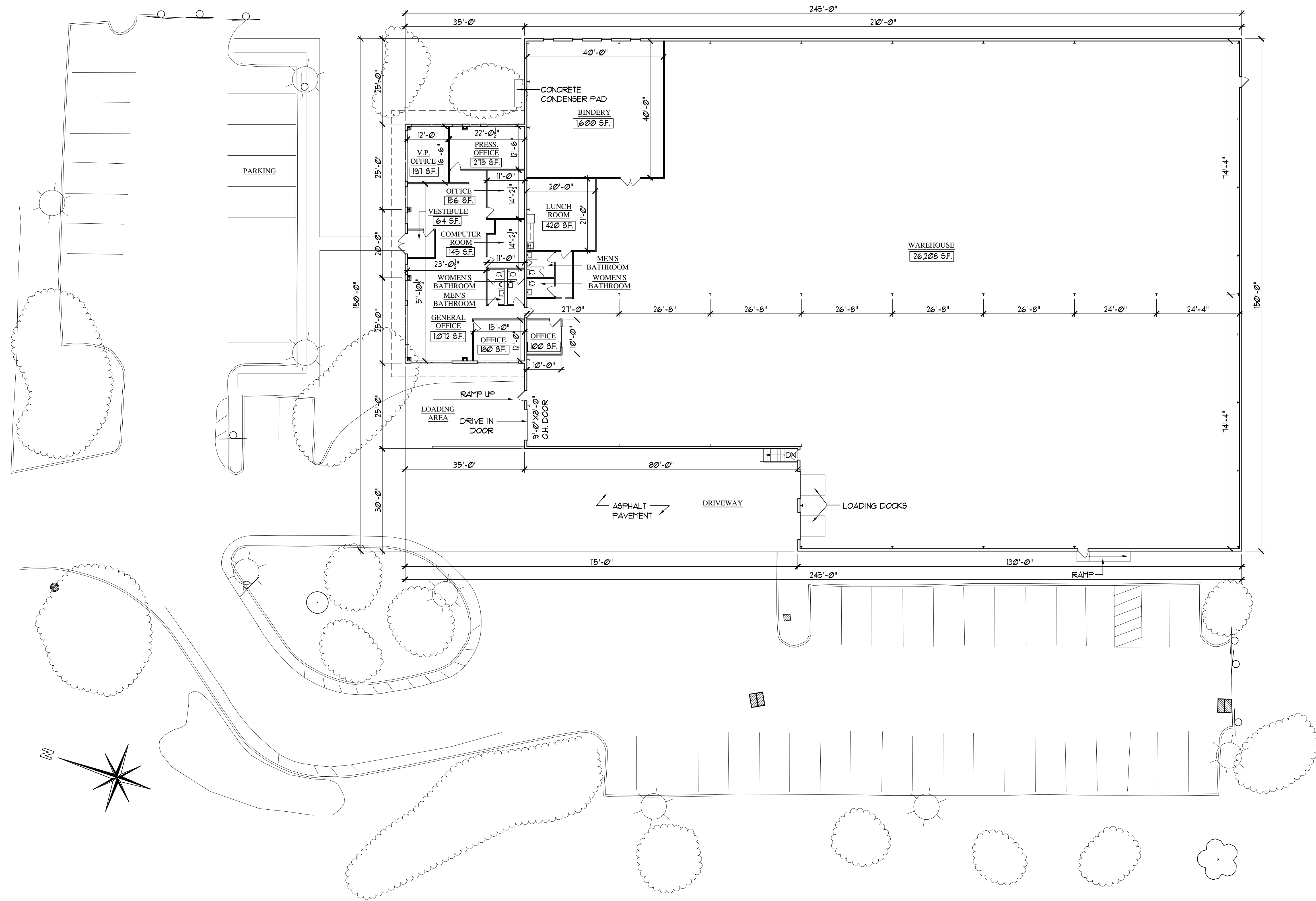
1 FLOOR PLAN 1/8" = 1'-0"
